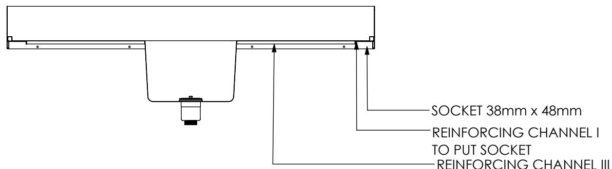
SECTION K-K
