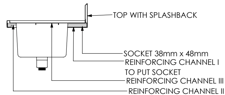
SECTION J-J
