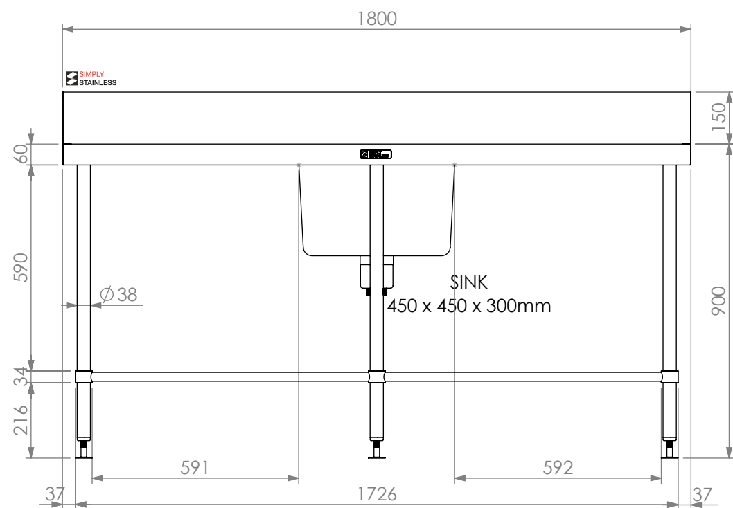
FRONT ELEVATION
