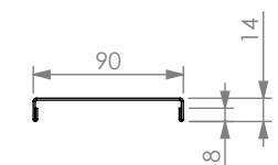
REINFORCING CHANNEL II DETAIL
