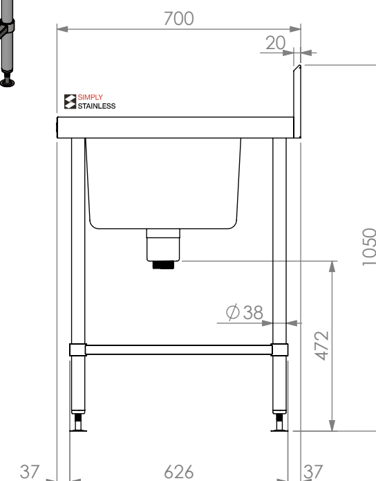
SIDE ELEVATION
