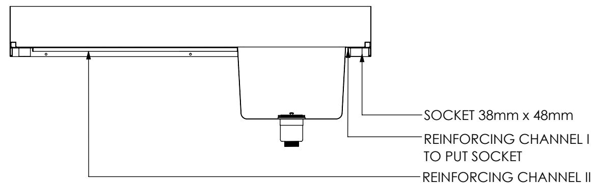
SECTION K-K
