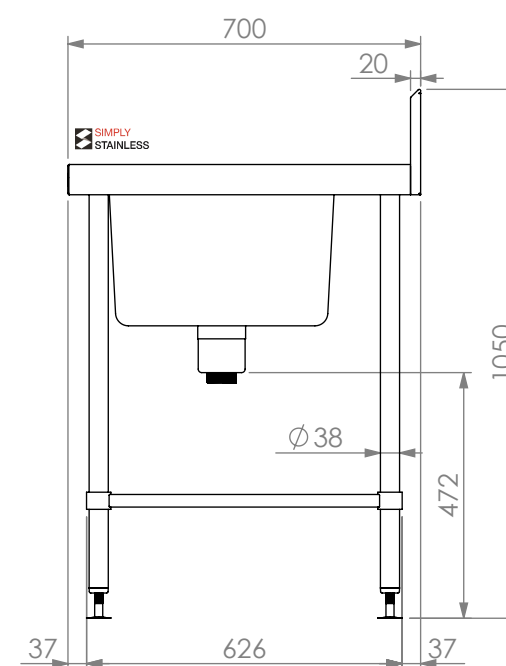
SIDE ELEVATION
