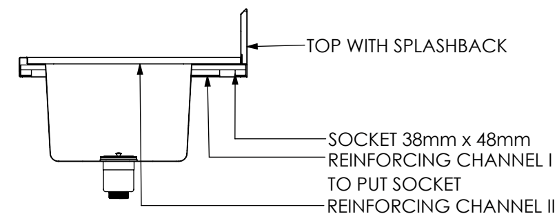
SECTION J-J
