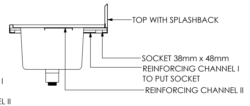
SECTION J-J
