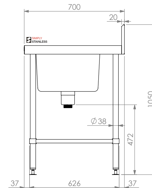
SIDE ELEVATION
