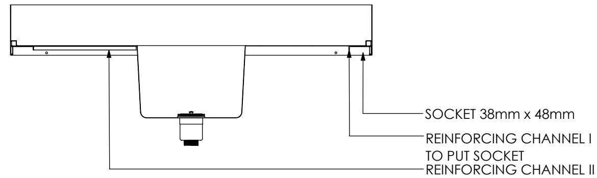
SECTION K-K
