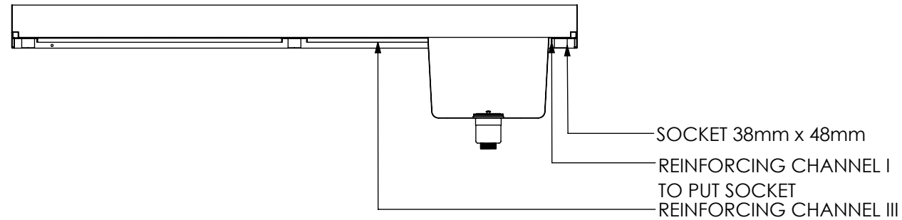
SECTION K-K
