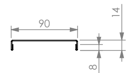
REINFORCING CHANNEL II DETAIL
