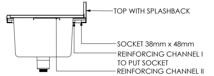
SECTION J-J
