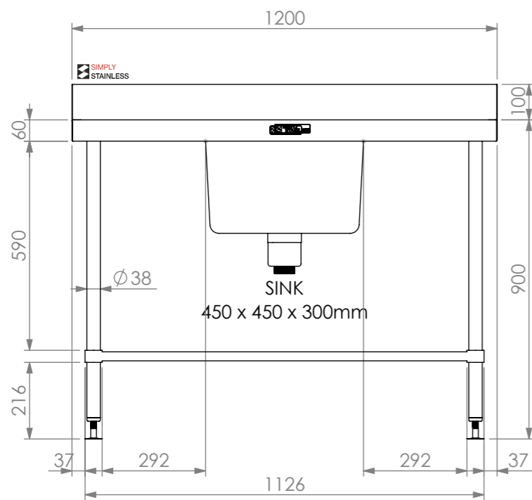
FRONT ELEVATION
