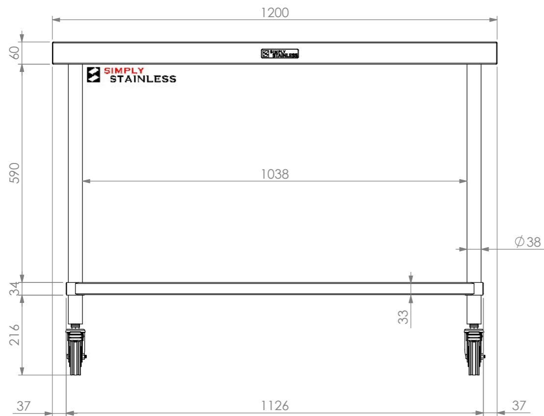
FRONT ELEVATION
