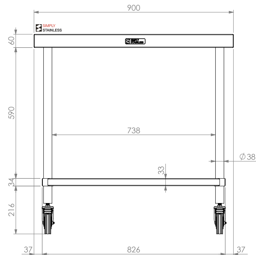
FRONT ELEVATION
