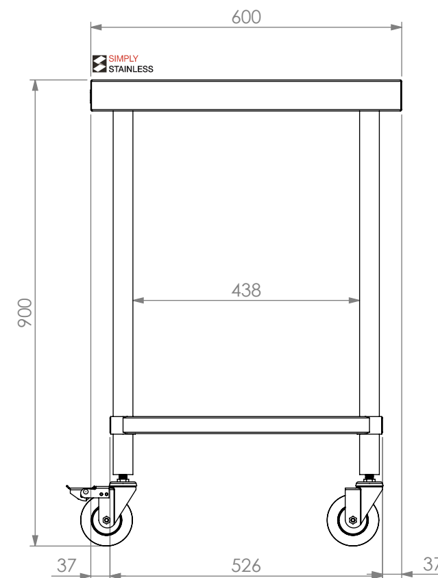
SIDE ELEVATION
