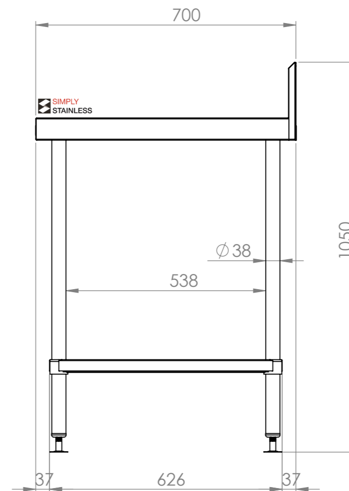
SIDE ELEVATION
