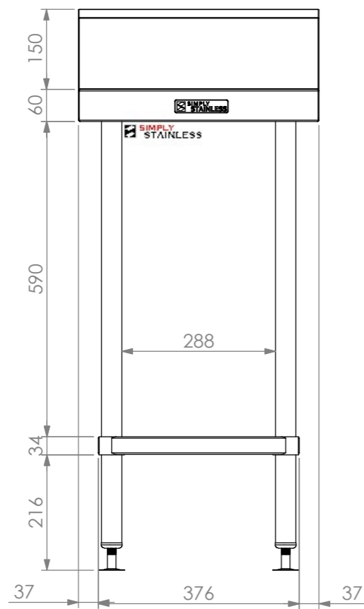
FRONT ELEVATION
