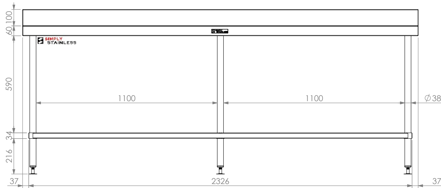
FRONT ELEVATION
