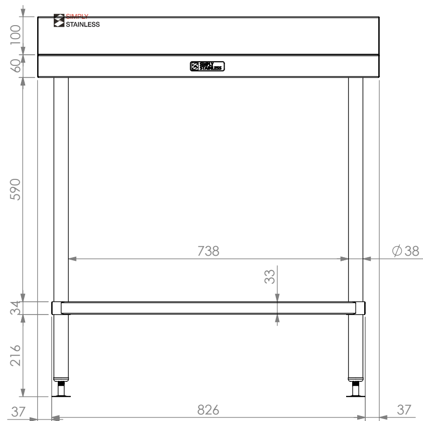
FRONT ELEVATION
