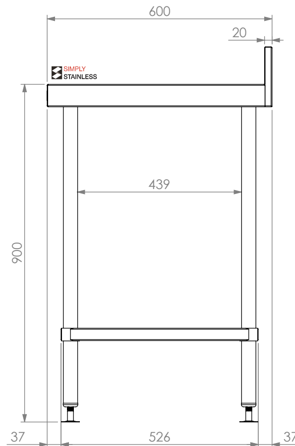
SIDE ELEVATION
