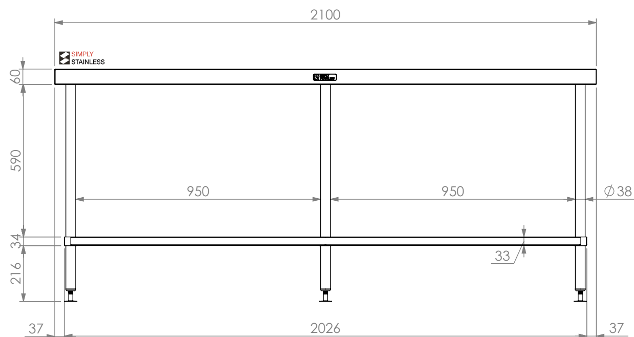
FRONT ELEVATION
