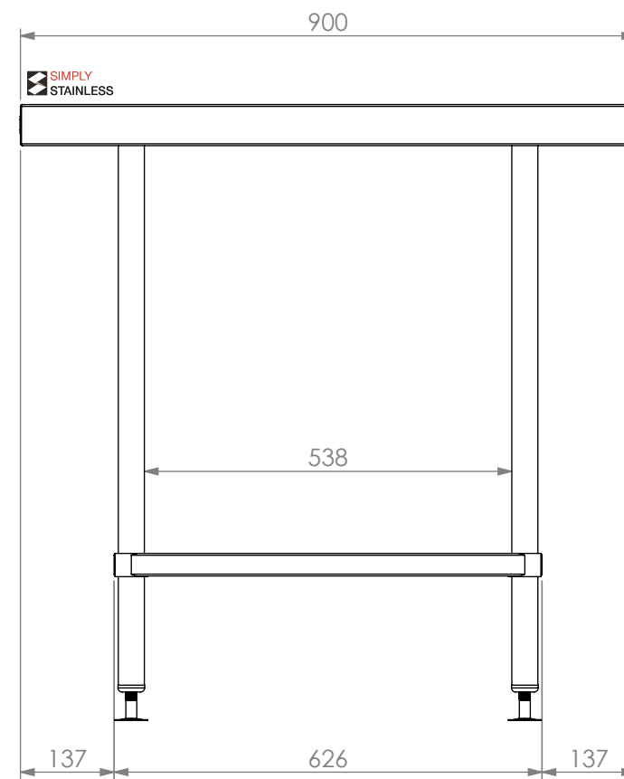
SIDE ELEVATION
