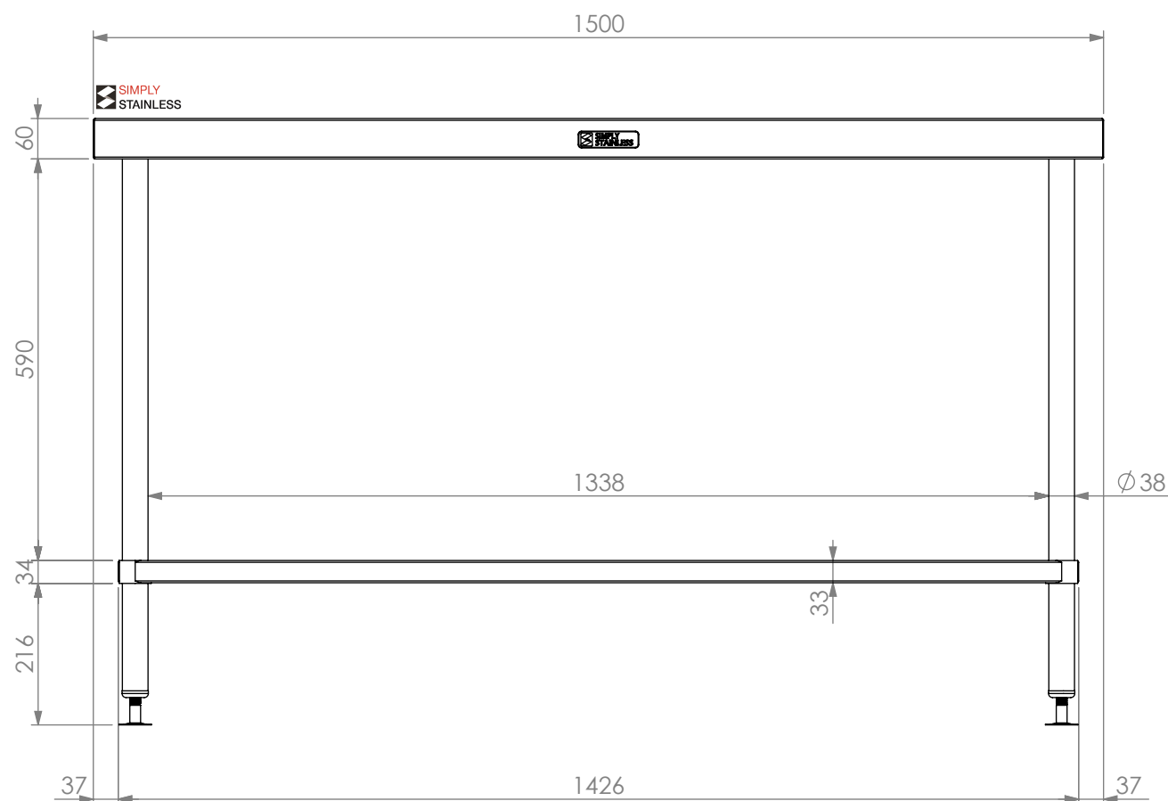
FRONT ELEVATION
