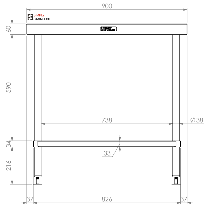
FRONT ELEVATION
