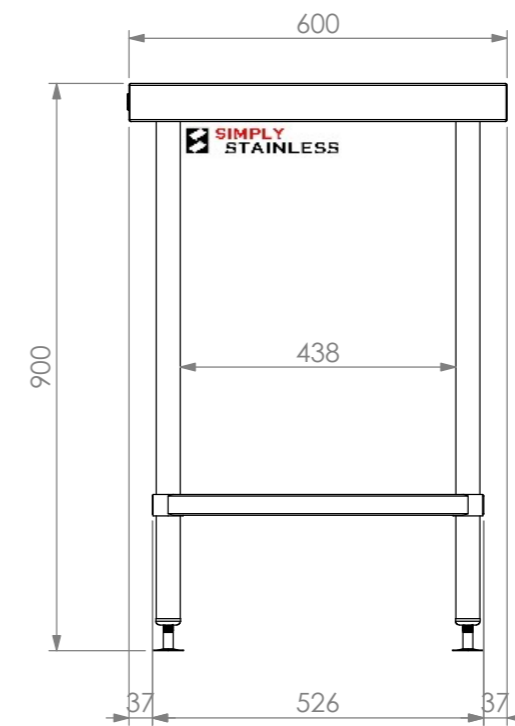
SIDE ELEVATION
