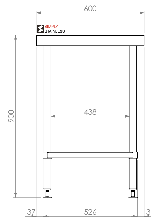
SIDE ELEVATION
