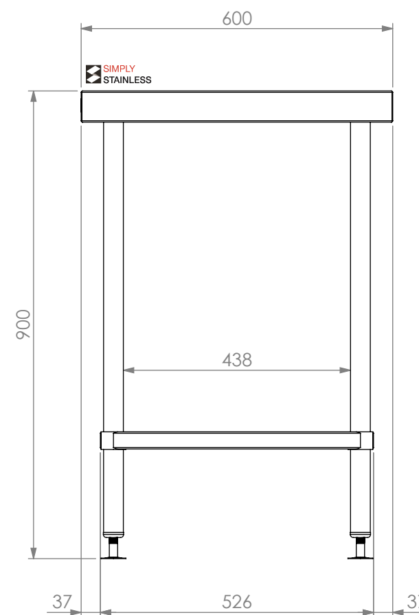
SIDE ELEVATION
