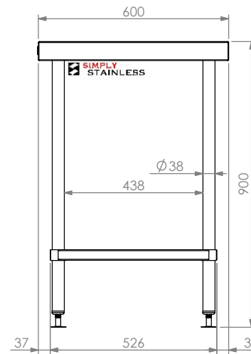
SIDE ELEVATION
