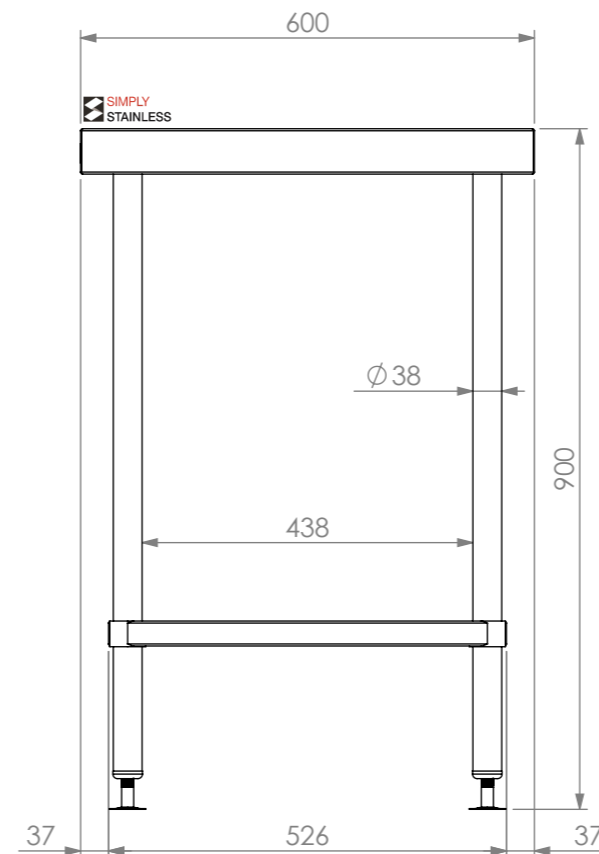
SIDE ELEVATION
