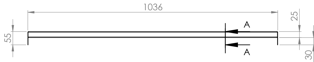
FRONT ELEVATION
