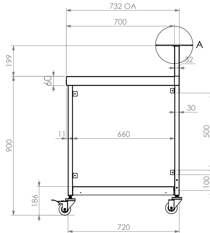
SIDE ELEVATION
