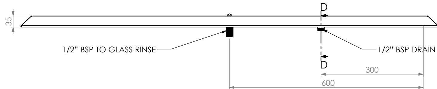
FRONT ELEVATION
