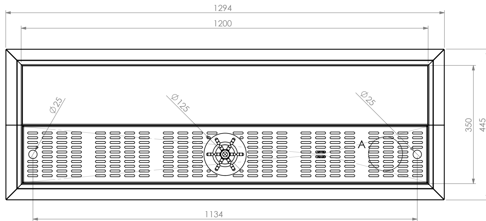
PLAN
