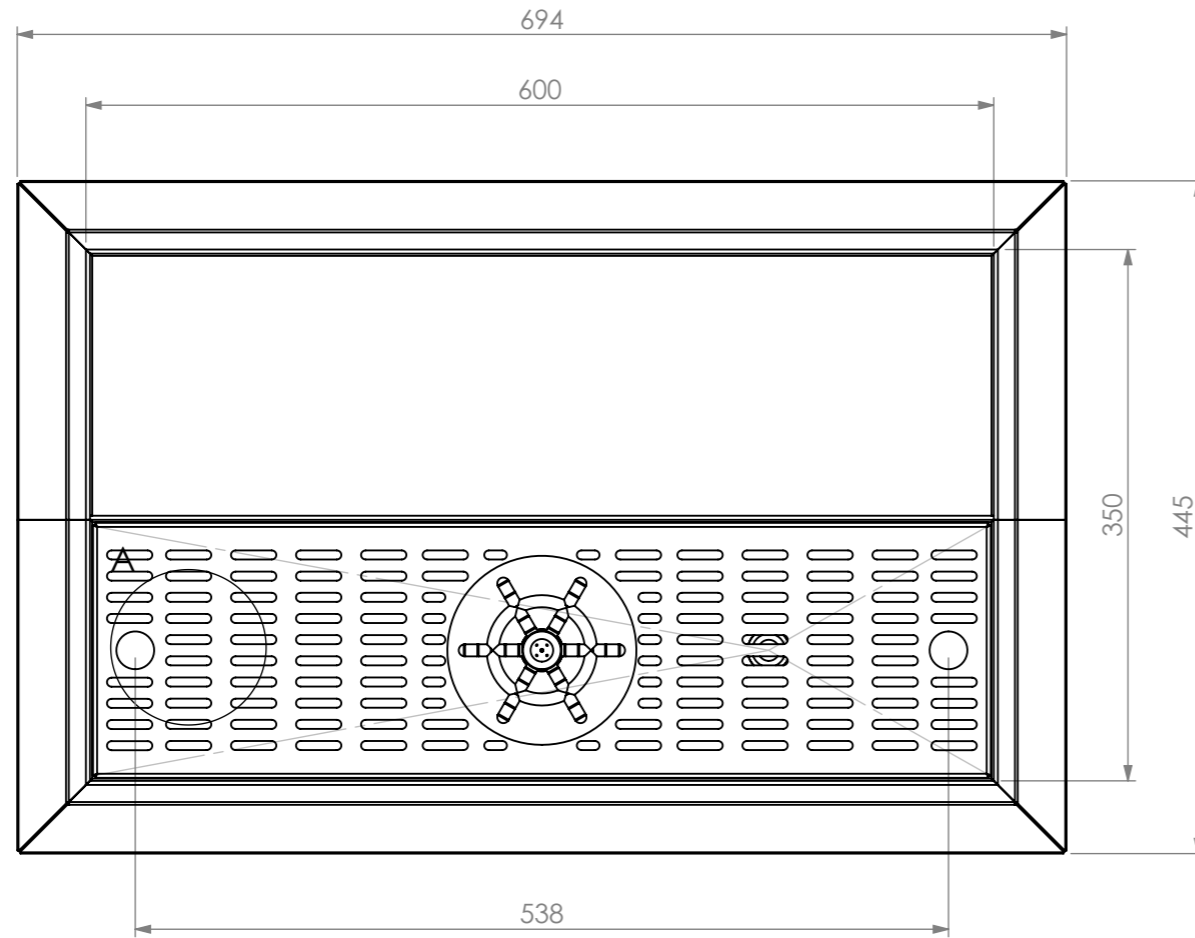
PLAN
