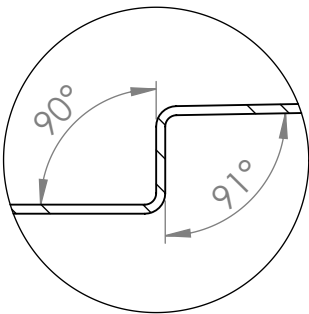
DETAIL E
