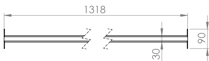
SPACER X1
