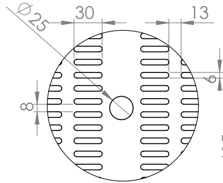
DETAIL C
