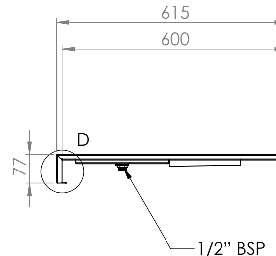
SIDE ELEVATION
