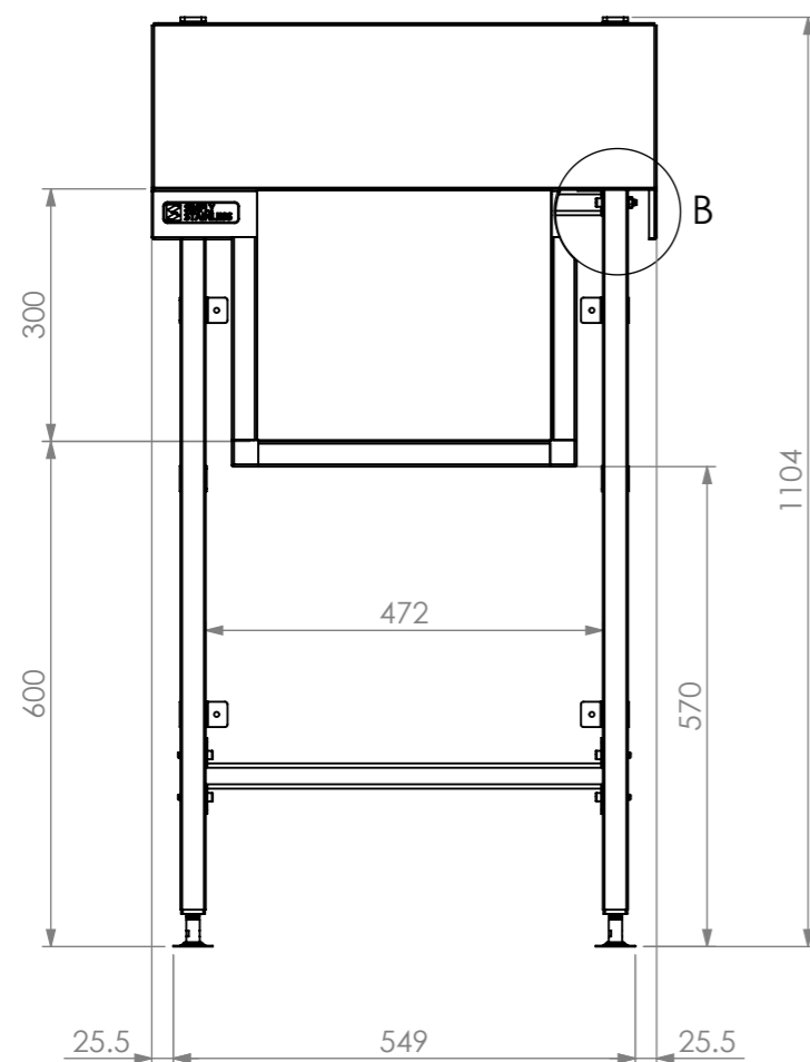
FRONT ELEVATION
