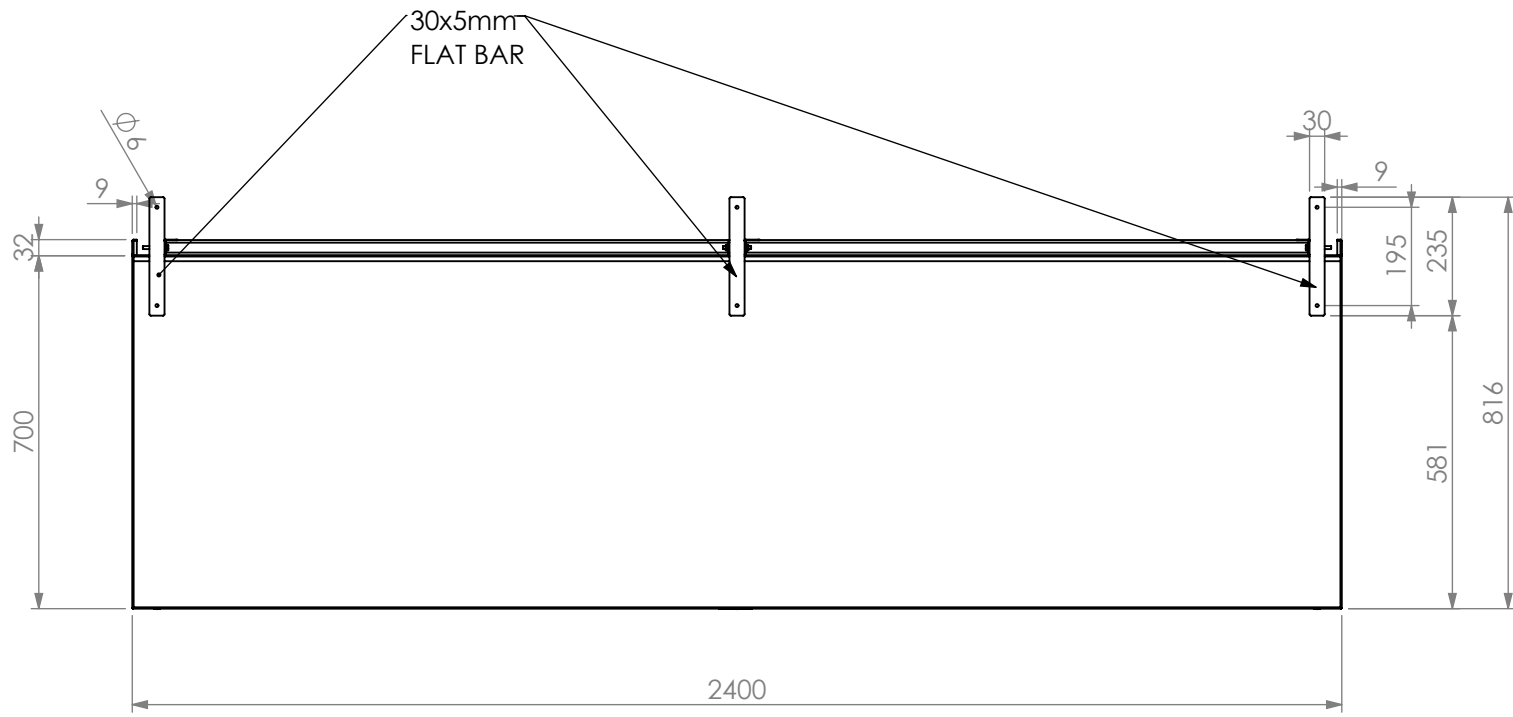
PLAN
