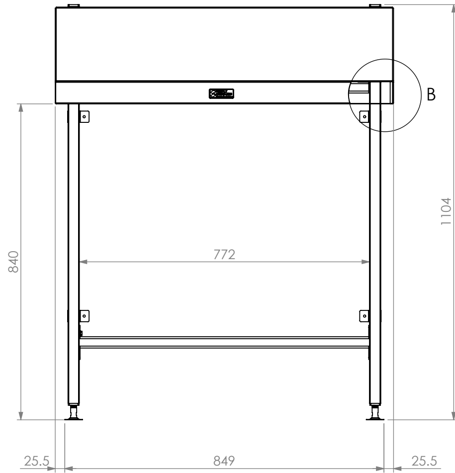
FRONT ELEVATION
