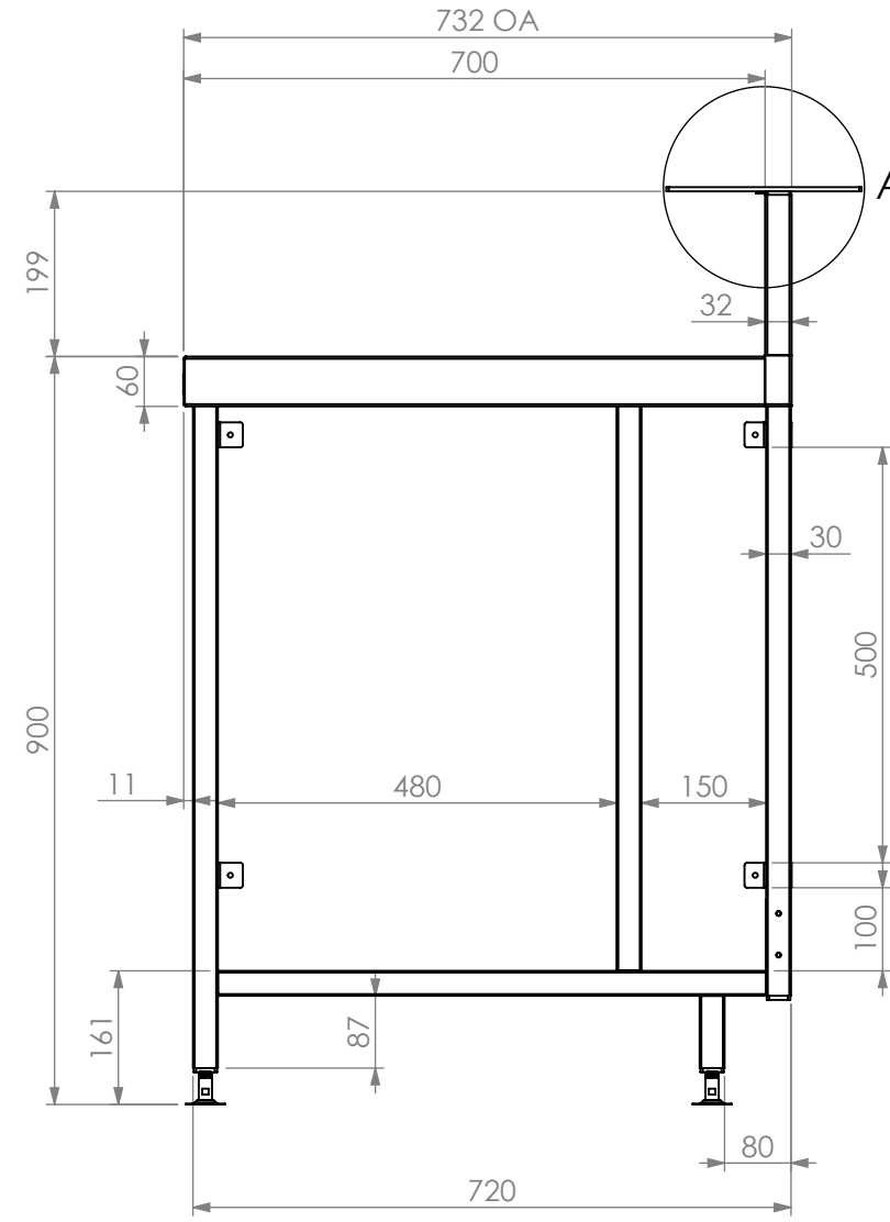
SIDE ELEVATION
