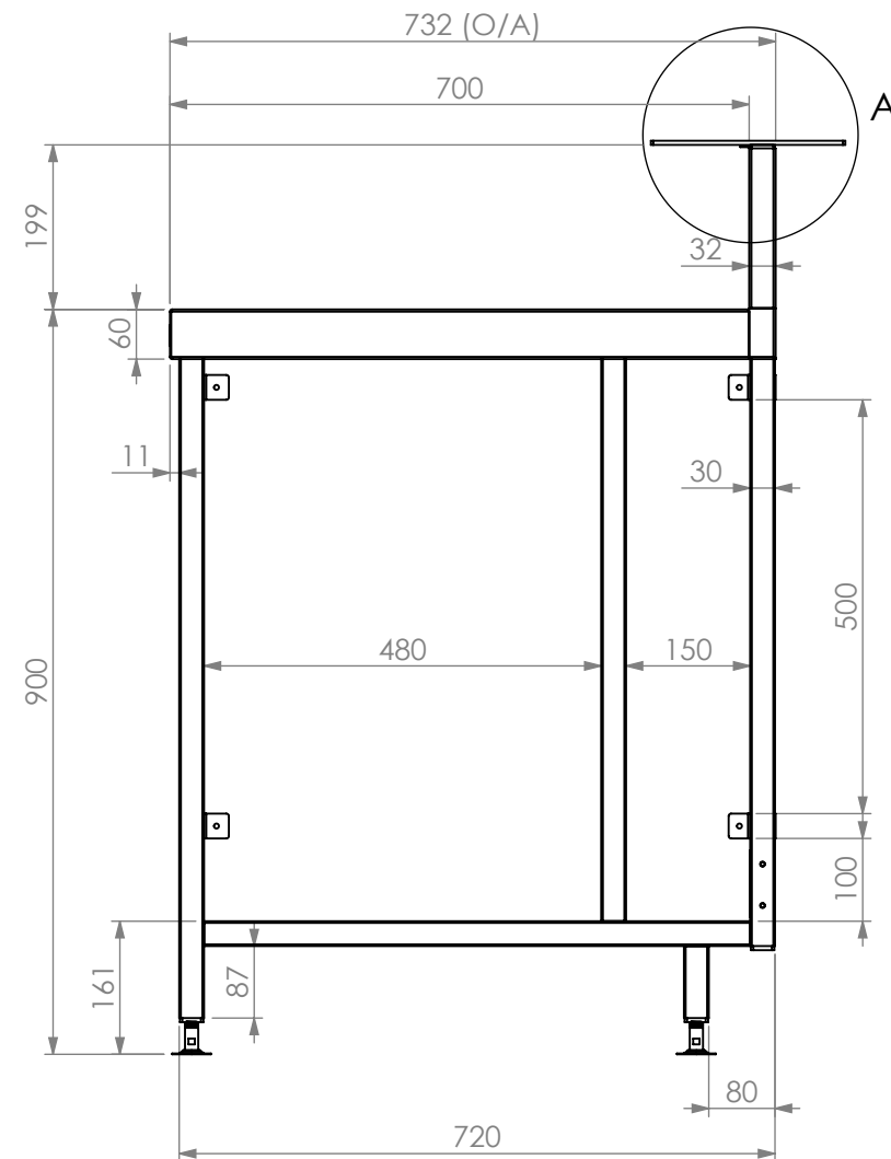
SIDE ELEVATION
