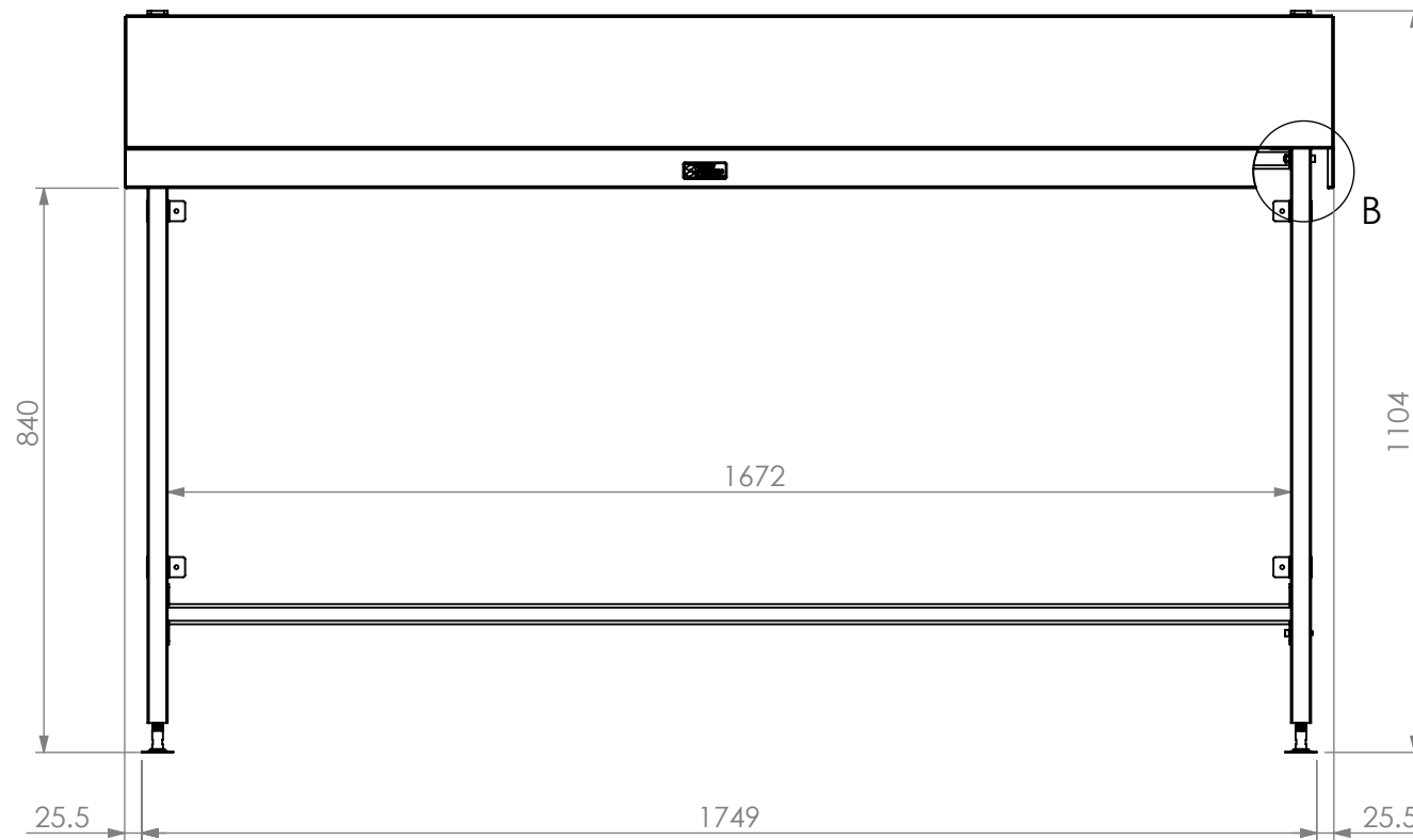
FRONT ELEVATION
