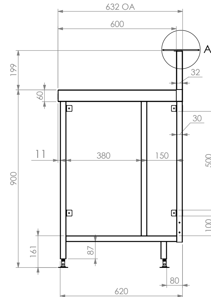
SIDE ELEVATION
