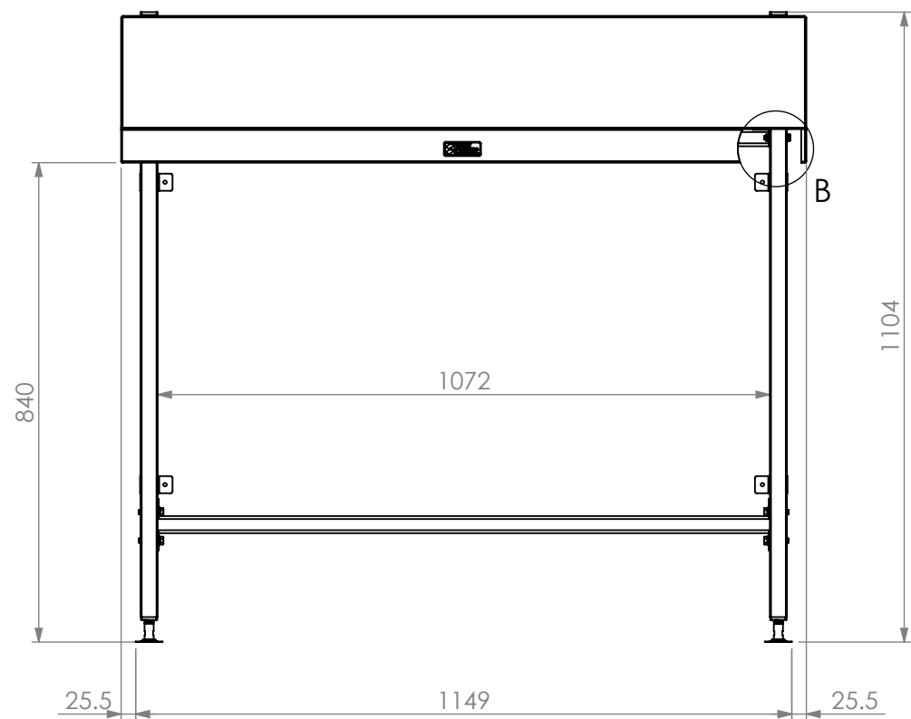
FRONT ELEVATION
