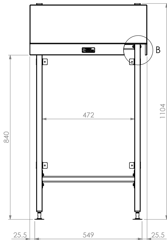
FRONT ELEVATION
