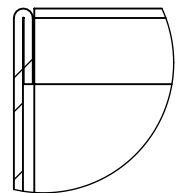
DETAIL B (SAFE EDGE TO TOP)
