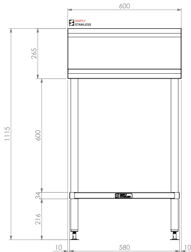
FRONT ELEVATION
