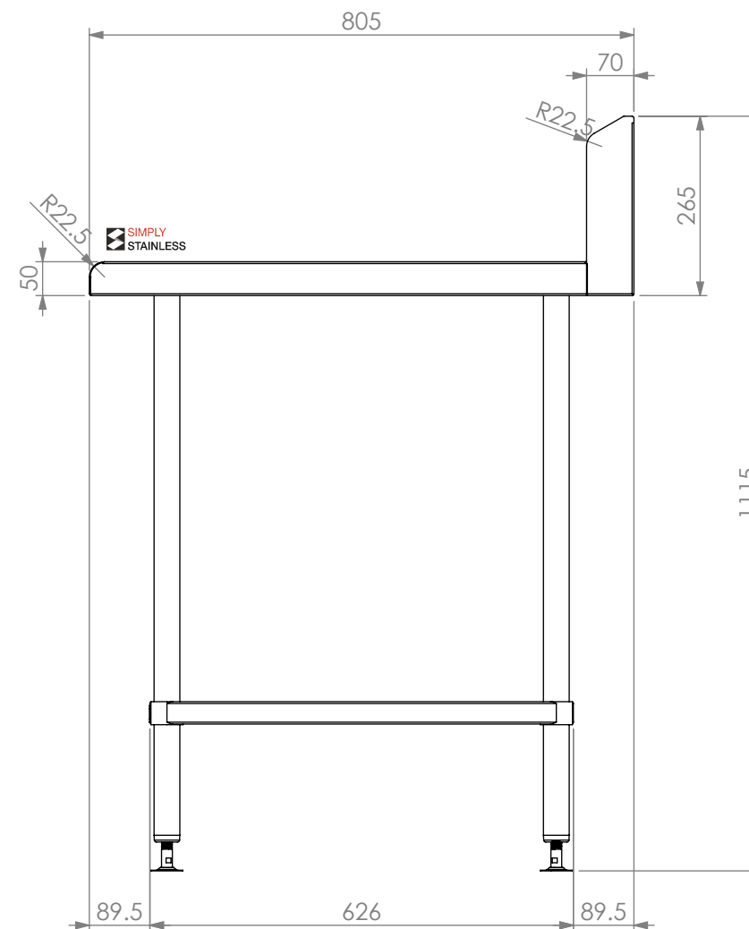
SIDE ELEVATION
