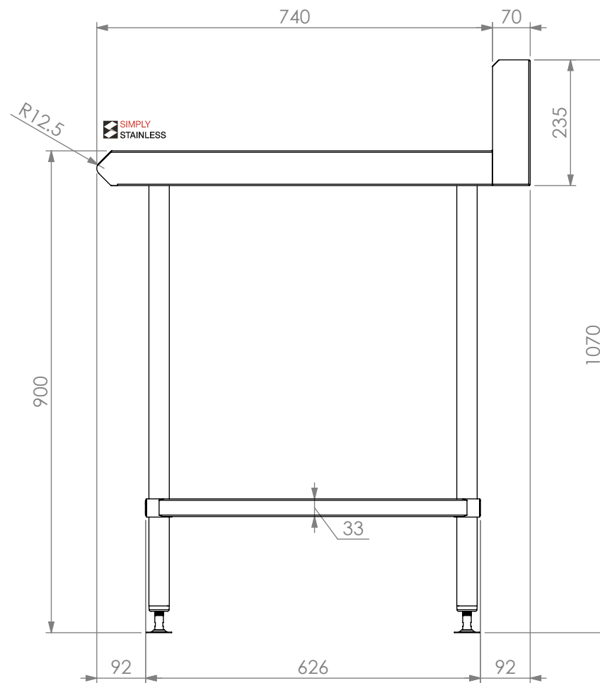
SIDE ELAVATION
