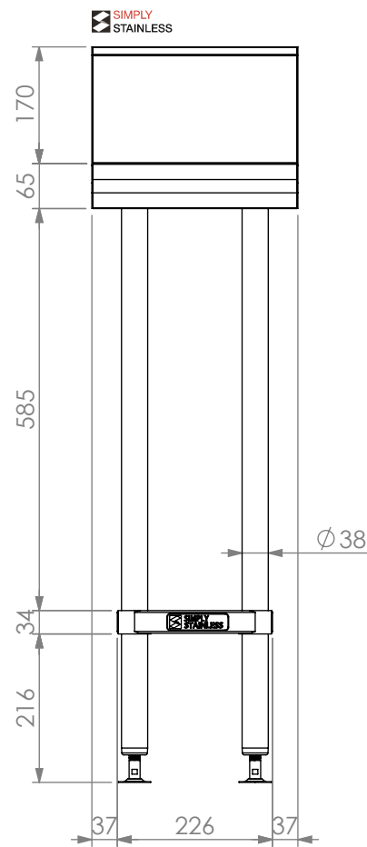
FRONT ELEVATION
