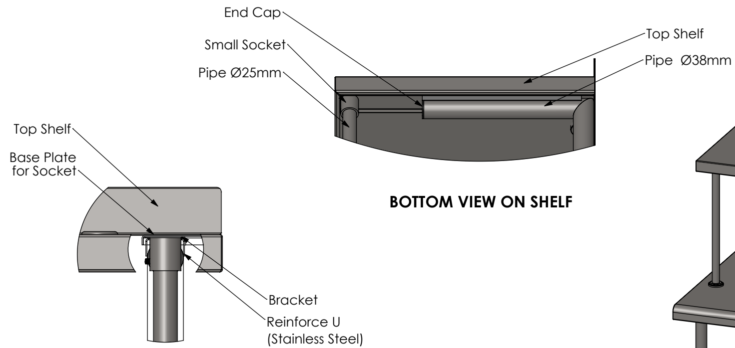
DETAIL A
