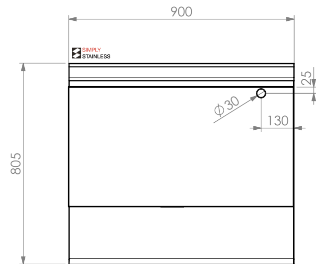
PLAN VIEW
