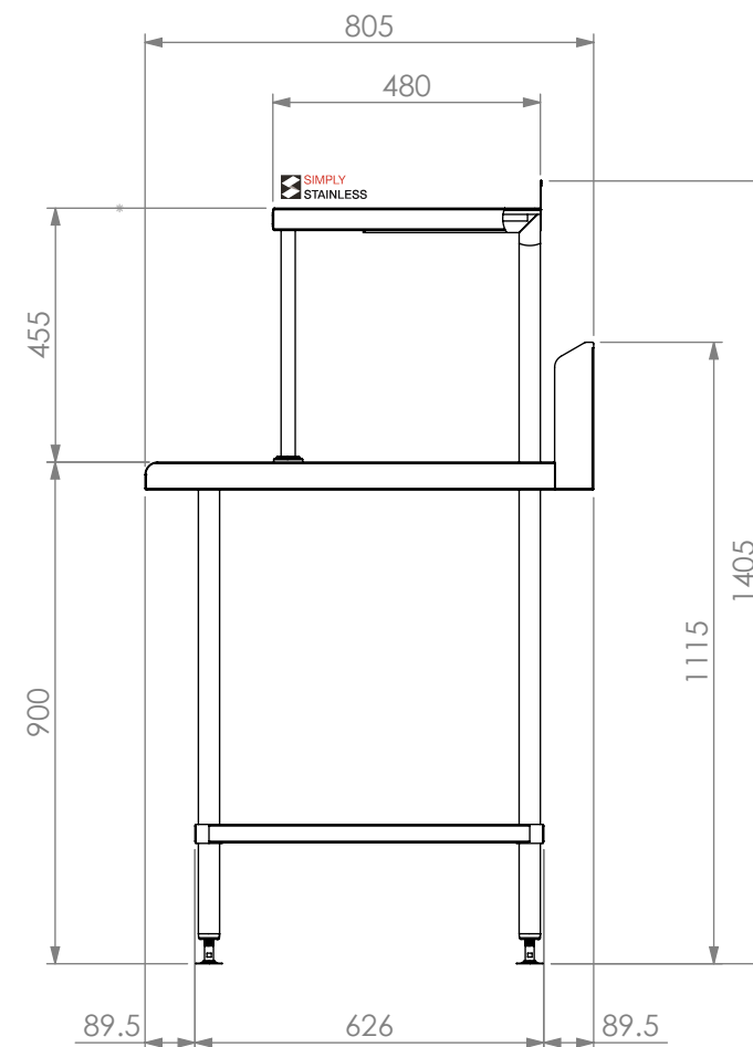
SIDE VIEW
