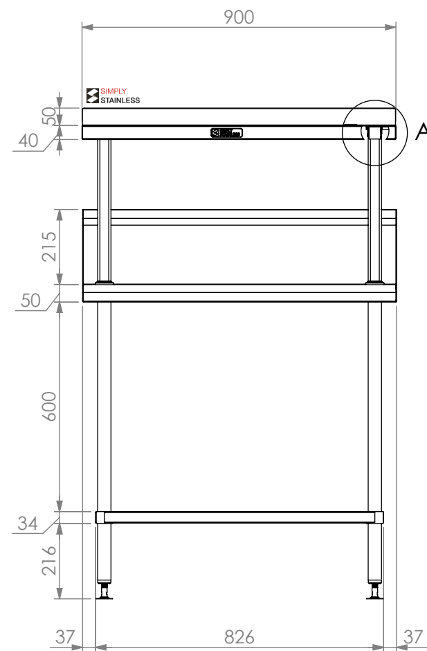
FRONT VIEW
