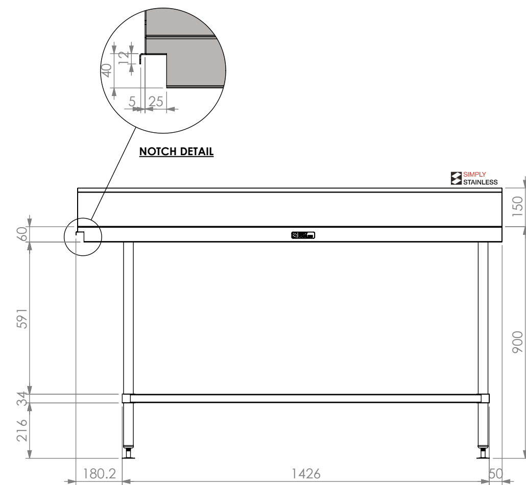
FRONT ELEVATION
