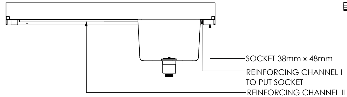
SECTION K-K
