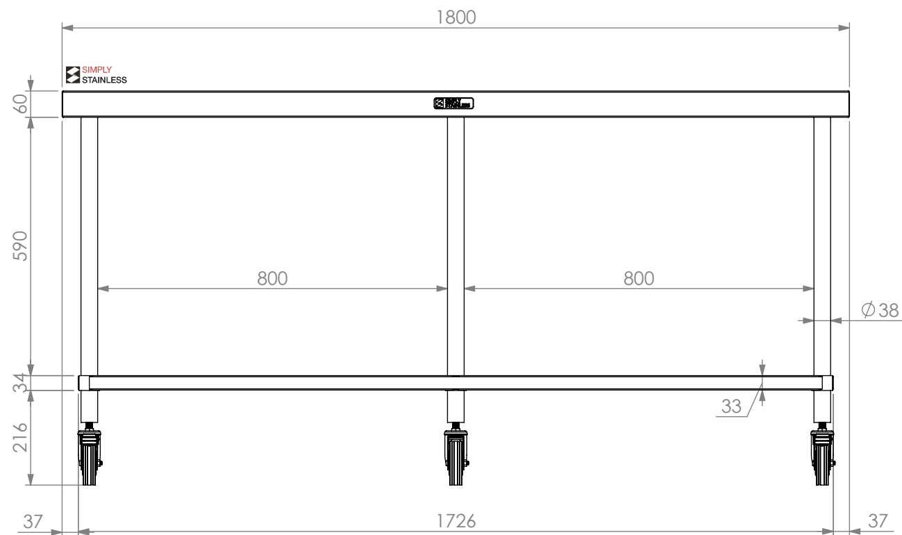
FRONT ELEVATION
