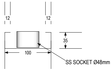
SECTION A-A Scale 1:5mm
