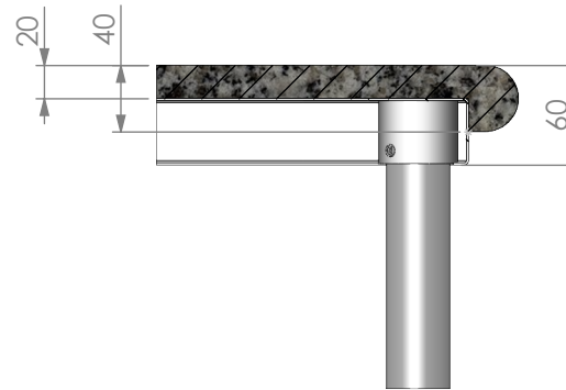
GRANITE TOP DETAIL
