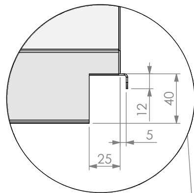
NOTCH DETAIL
