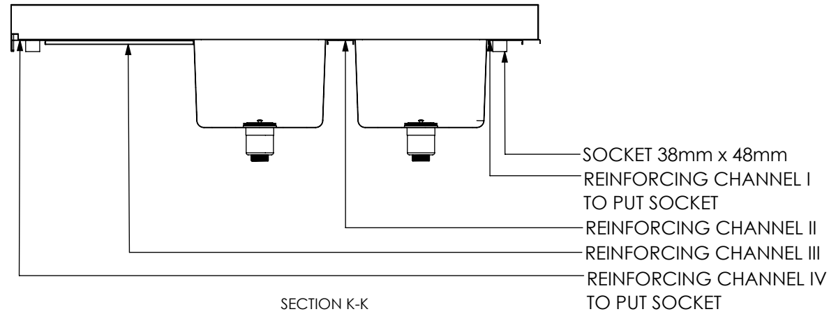
SECTION K-K
