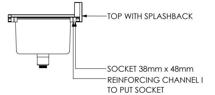
SECTION J-J
