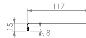
REINFORCING CHANNEL I DETAIL
