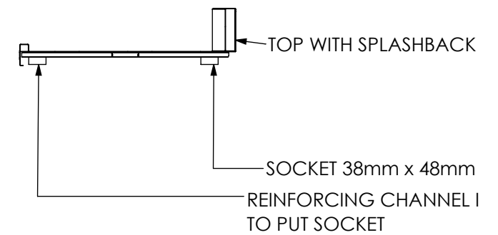
SECTION J-J
