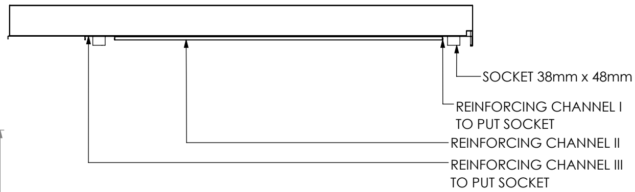
SECTION K-K
