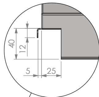
NOTCH DETAIL
