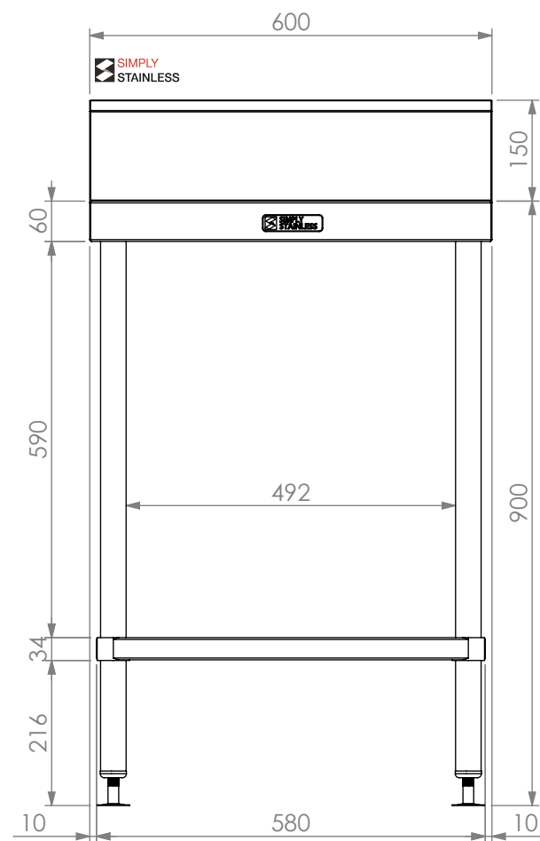
FRONT ELEVATION
