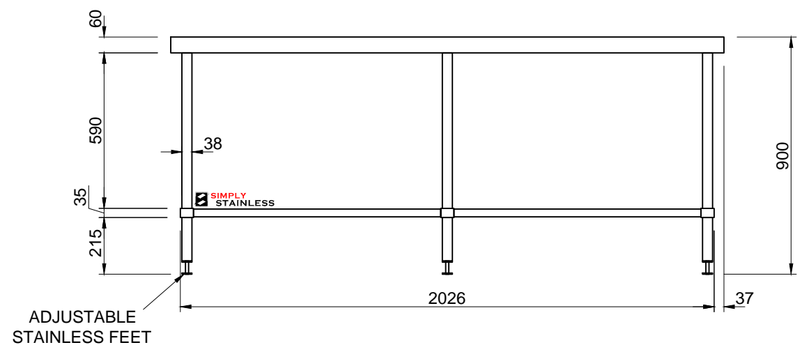
FRONT ELEVATION
